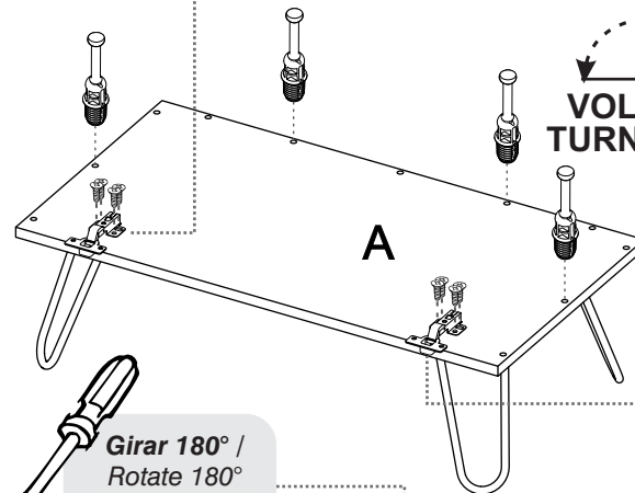
Bisagra Interior/ Half overlay hinge
